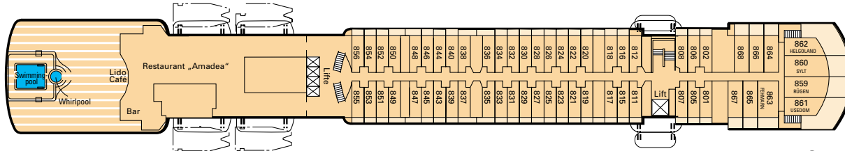
PROMENADEN-DECK (Deck 7)
